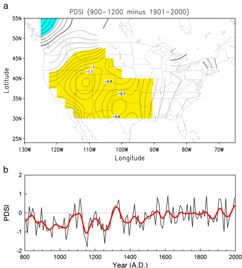
Fig. 1. (a) Difference in tree-ring reconstructed PDSI for 900–1200 AD minus 1901–2000. Negative values indicate the regions were drier in MT. Shadings indicate the differences are significant at 95% confidence level by two-tailed Student t -test. (b) Regional averaged PDSI for the western U.S. (30–50°N, 90–125°W). To retain the low frequency variations in PDSI, only the 10-yr average values of PDSI were shown. The red lines show the low frequency variations of PDSI by low pass binomial filter. (adapted from Feng et al., 2008).
