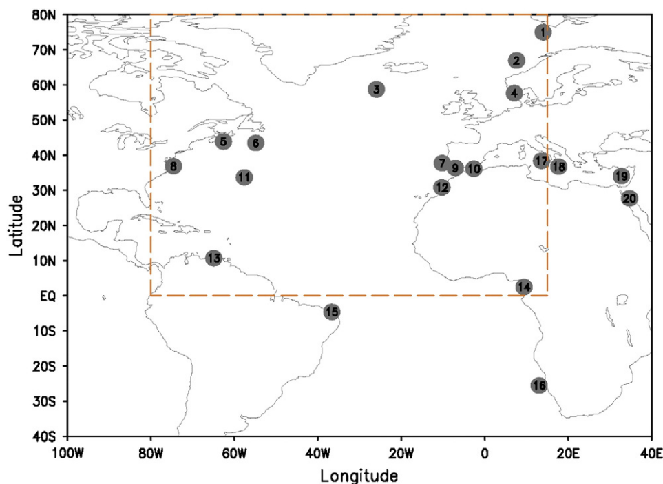
Fig. 4. Spatial distribution of the proxy SST records used in this study. The (numbered) gray dots in the Atlantic Ocean mark the 20 sites where proxies for SST were obtained (details of those sites and the temporal SST variations in individual site are shown in Feng et al. (2009)). Dashed rectangle shows the regions dominated by basin-wide AMO signal during the instrumental period.
