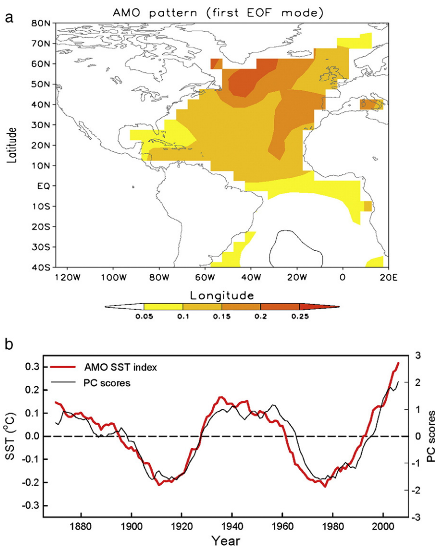
Fig. 2. Observed summer (June–August) SST pattern associated with AMO and the temporal variations of the AMO index. (a) The first EOF of the SST in the North Atlantic Ocean. Before EOF analysis, the SST in each grid point was first detrended and then smoothed with a 9-point equal-weight low pass filter. (b) Temporal variations of the first principal component (PC) associated with the EOF mode (black line), and the regional averaged summer detrended SST anomalies (red line) over the North Atlantic Ocean (0–60°N, 7.5–75°W).
