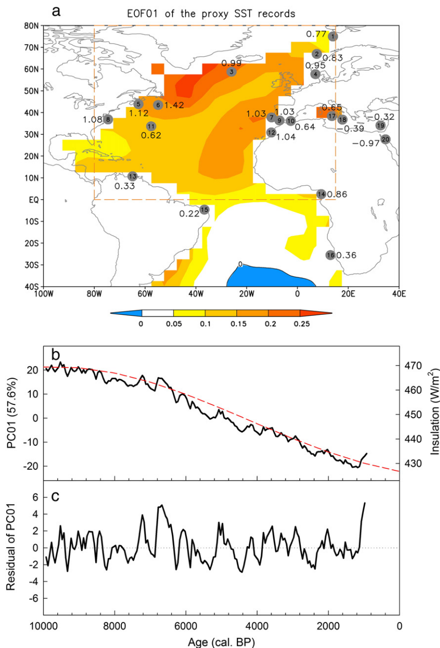
Fig. 5. EOF results of the proxy SST records. (a) Spatial distribution of the first EOF. The (numbered) gray dots show the 20 sites where proxy SST records were obtained (see Fig. 4). The value by each site is the eigenvector of the first EOF of the proxy SST record. (For illustration purposes, shading shows the first EOF of the observed summer SST in the North Atlantic Ocean on decadal and longer timescales, essentially the AMO pattern as defined from observations. The decadal and longer time-scales variations in detrended summer SST are smoothed using a 9-year equal-weight filter, which remove the SST variations shorter than 9 years.). Dashed rectangle shows the regions dominated by basin-wide AMO signal during the instrumental period. (b) PC01 of the 20 proxy SST records (thick line) and July insolation at 65°N during the Holocene (dashed line). (c) Detrended time series of PC01. Details of the results can be found at Feng et al. (2009).
