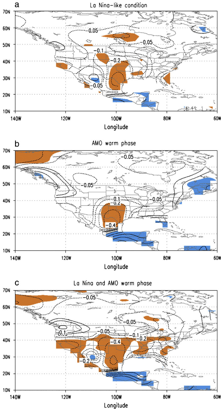
Fig. 3. Influences of (a) La Niña-like condition in eastern tropical Pacific Ocean, (b) AMO warm phase SST in the North Atlantic and (c) both La Niña-like SST in the tropical Pacific and AMO warm Phase SST in the North Atlantic on the annual averaged daily precipitation (mm/day). Detail of those model simulations can be found at Feng et al. (2008) .
